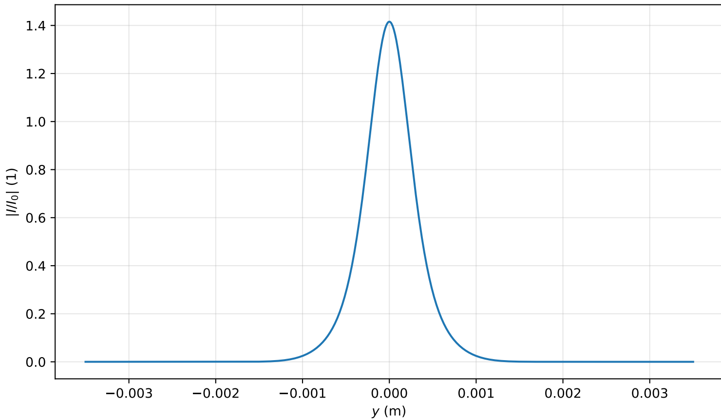
Intensity profile I(x=0, y, z=1.035)/I_0 , \text{Pin}=0.9\text{Pcr} , artificial time
